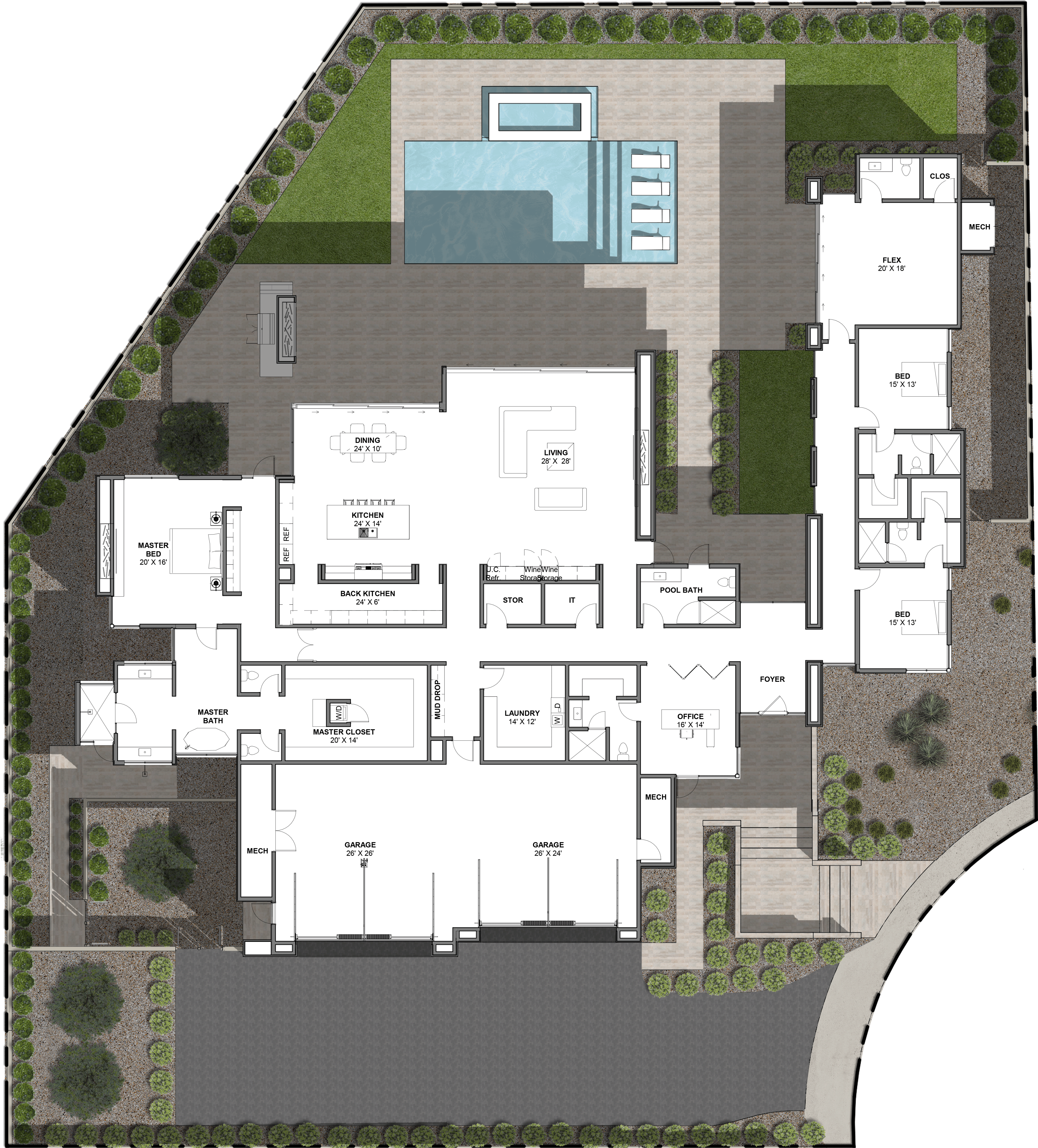
1 LOT 2 - CONCEPTUAL SITE PLAN 1" = 20'-0"
