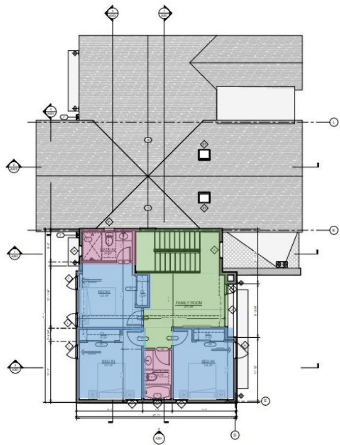
2 LEVEL 2 1" = 4'-0"
