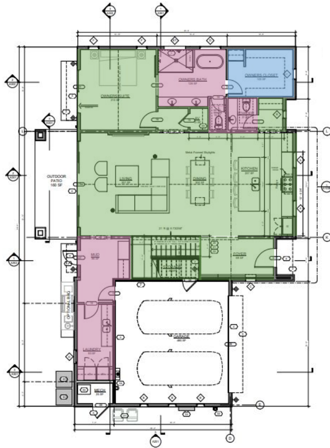
1 LEVEL 1 1" = 4'-0"
